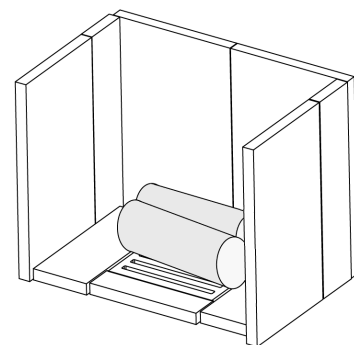
How to lay firewood in combustion chamber of W14, W14A, W14K, W14R
